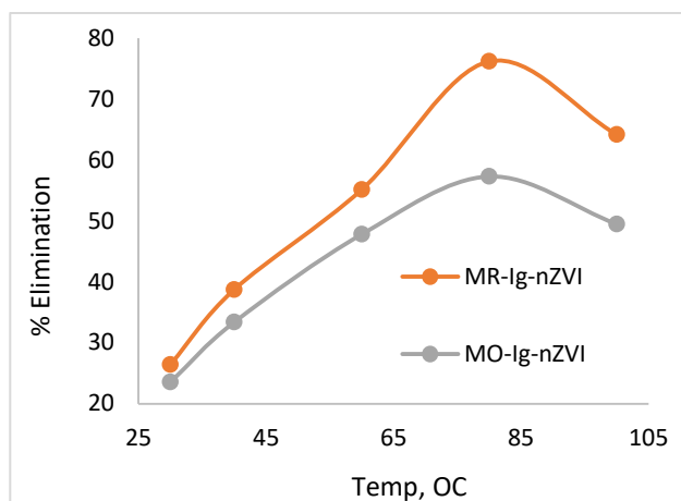
Figure 6: Effect of Temperature on removal of MR with Ig-nZVI
