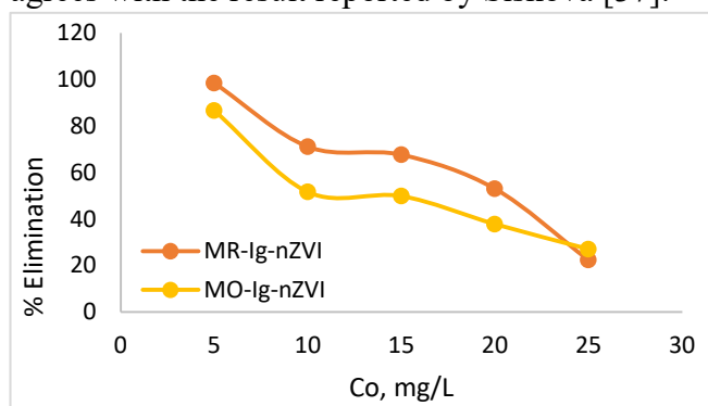
Figure 3: Effect of Initial Concentration on removal of MR and MO with Ig-nZVI
