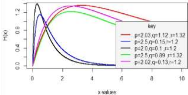
Figure 8: Hazard rate plot for some selected values of parameters of TELTL-W
