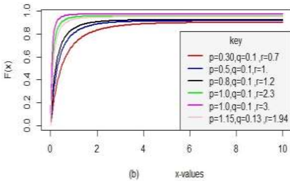
Figure 2: cdf plot for some values of parameters of TELTL-E
