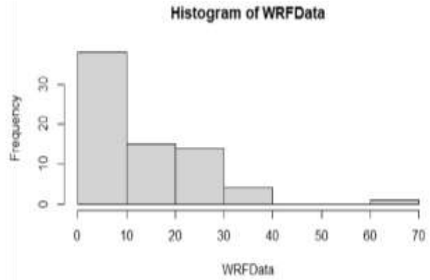
Figure 11: Histogram showing the skewness of Wheaton River flood data sets.
