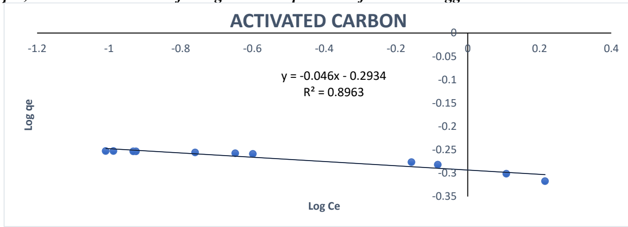
Figure 9: Freundlich adsorption isotherm for Cadmium (II) ions removal at a speed of 150 rpm, neutral pH, initial concentration of 20mg/L and temperature of 25°C with activated carbon.
