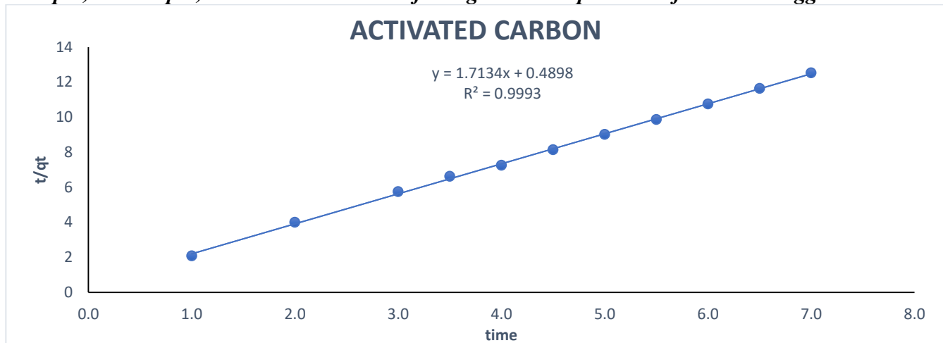
Figure 13: pseudo-second order (Ho) kinetic model plot of Cadmium (II) ions adsorption at a speed of 150 rpm, neutral pH, initial concentration of 20mg/L and temperature of 25°C with activated carbon
