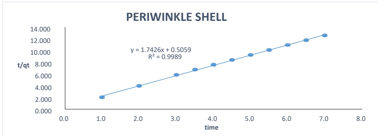
Figure 10: pseudo-second order ( H_0 ) kinetic model plot of Cadmium (II) ions adsorption at a speed of 150 rpm, neutral pH, initial concentration of 20mg/L and temperature of 25°C Periwinkle Shell.
