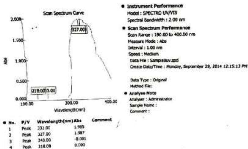
UV spectrum of isolate A
