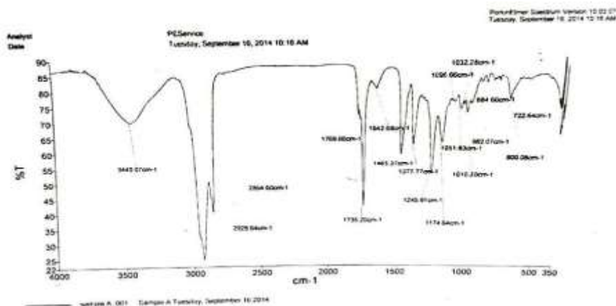
IR spectrum of isolate A
