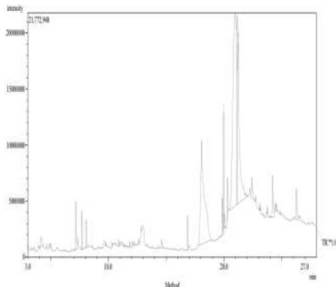
Figure 6: GC-MS spectrum of methanolic fruit extract of Thespian garckeana
