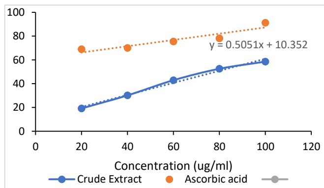
Figure 3: DPPH scavenging activity of Thespian garckeana fruit extract against ascorbic acid
