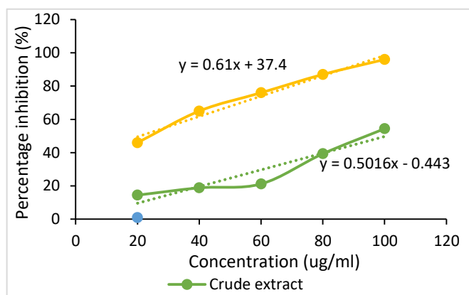
Figure 4: Total Antioxidant Capacity of Thespian garckeana fruit extract against ascorbic acid
