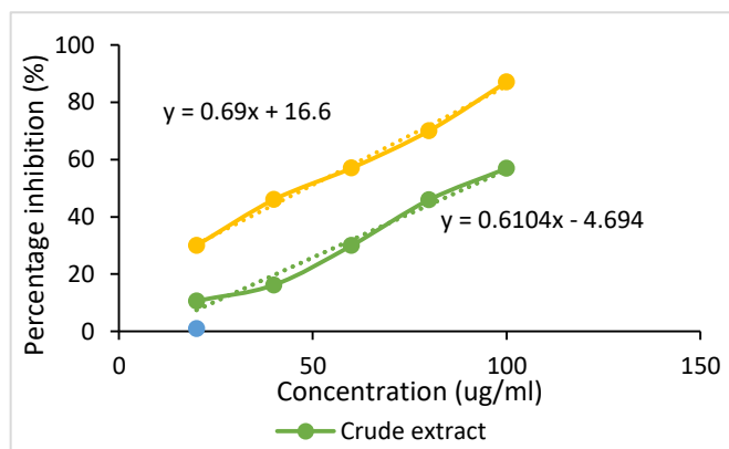
Figure 5: Nitric oxide scavenging activity of Thespian garckeana fruit extract against ascorbic acid
