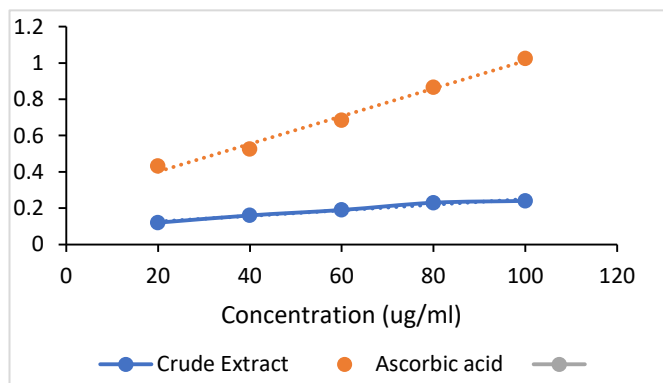
Figure 2: Reducing power activity of Thespian garckeana fruit extract plotted against ascorbic acid (standard).
